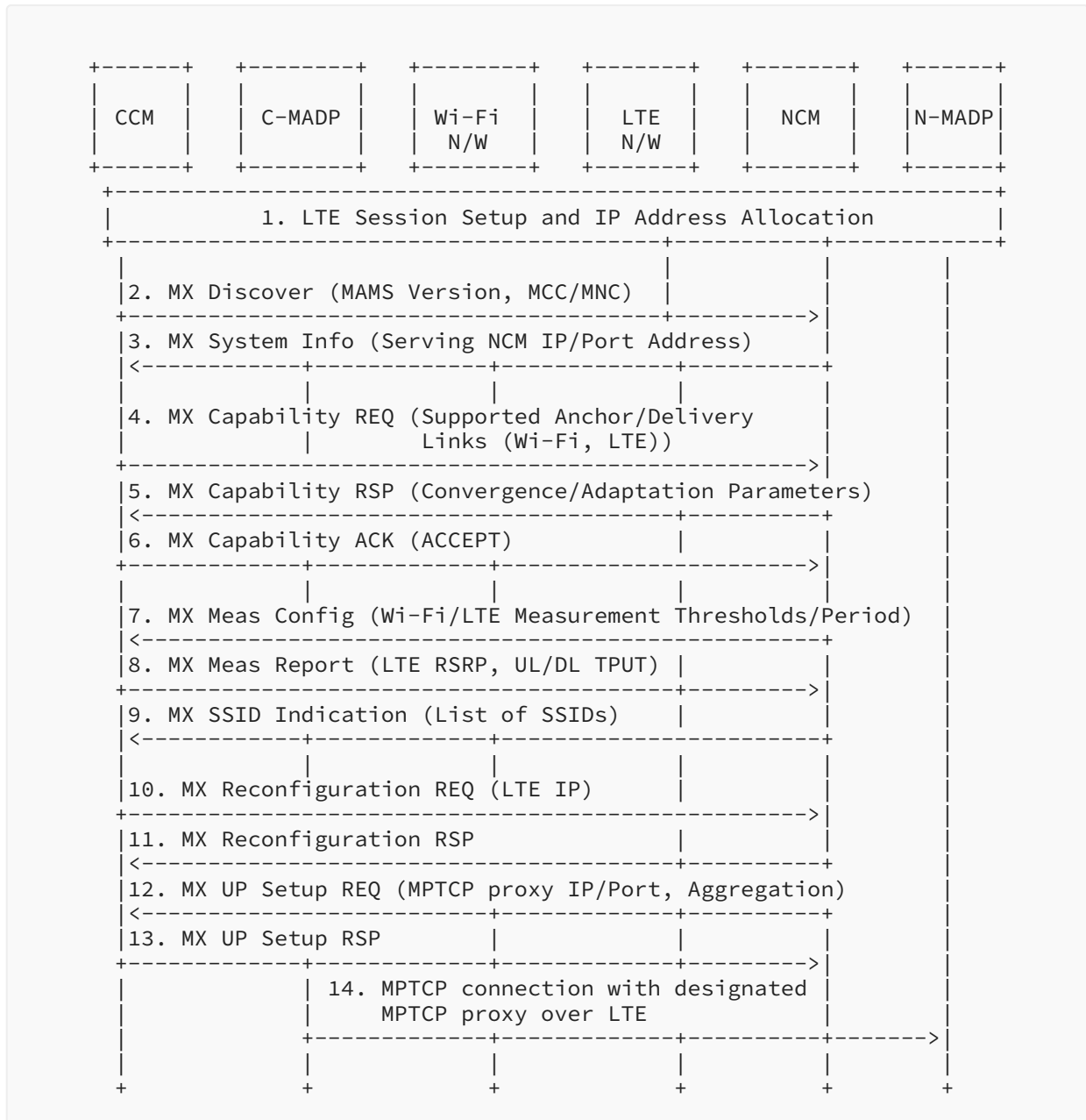
Figure 18: MAMS-Assisted MPTCP Proxy as User Plane - Initial Setup with LTE Leg
